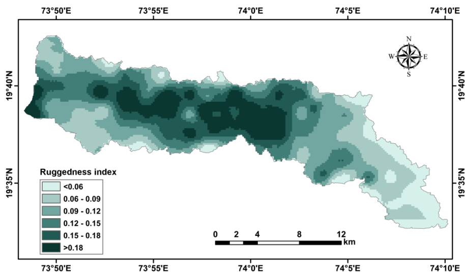
Figure 11. Ruggedness index
