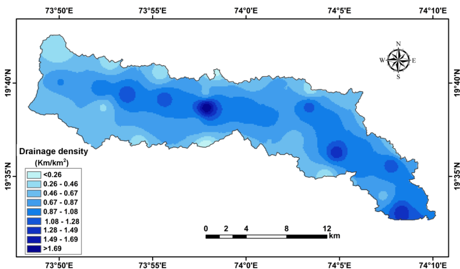
Figure 4. Drainage density
