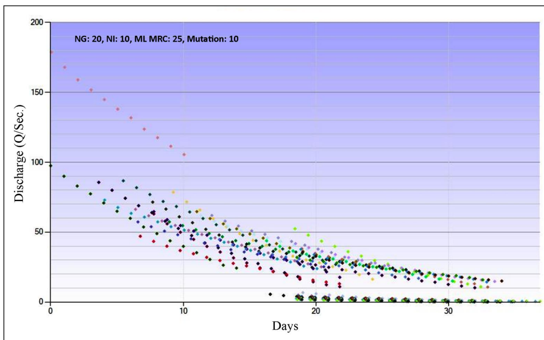
Figure 3. Visualization of the best solution for optimization of MRC-genetic algorithm
