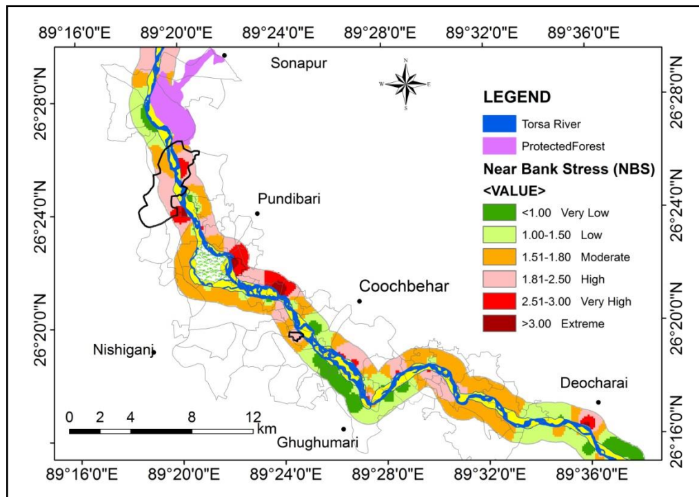
Figure 5. Near bank stress rating zones
