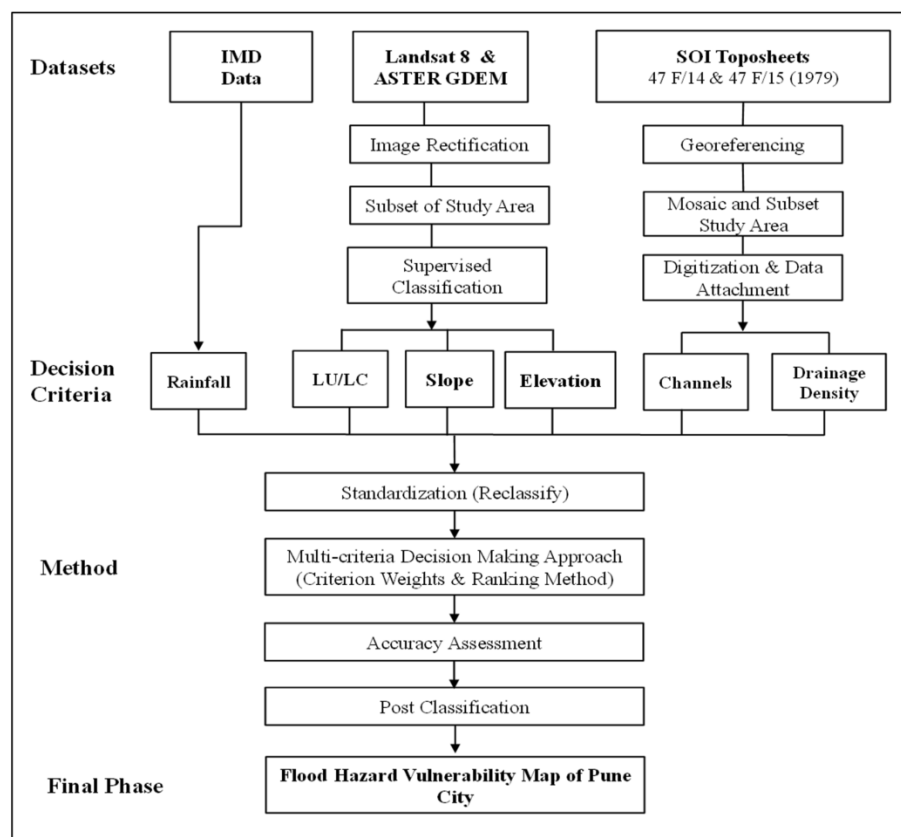
Figure 2. Methodology
