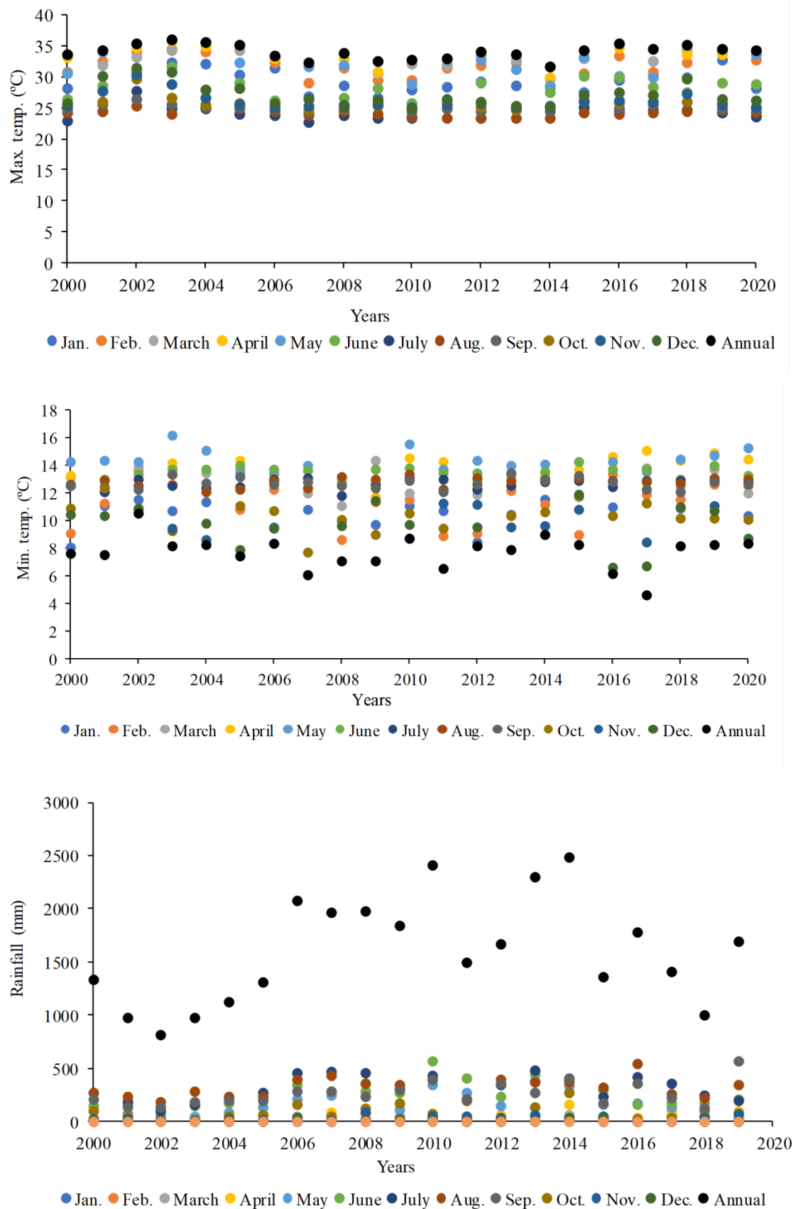
Figure 9. Temperature and rainfall during 2000-2020
