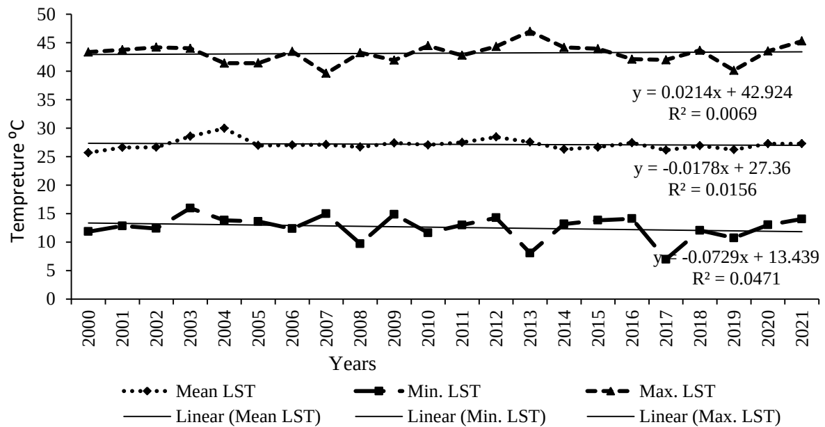
Figure 11. LST from MODIS data (2000-2021)
