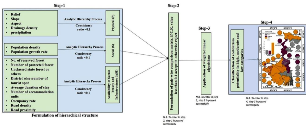
Figure 2. Methodology
