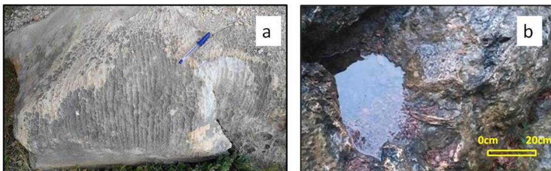
Figure 6. a) A general view of rillen karren in Darnah Formation and b) Solution basins in Darnah Formation.
